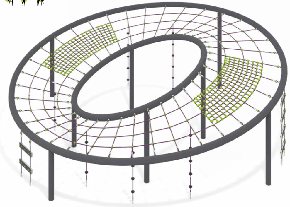
21.019 Rope Climbing Playground Baikal width length height fall height 6 170 mm 6 250 mm 2 100 mm 2 100 mm Age range: 7-12 years
