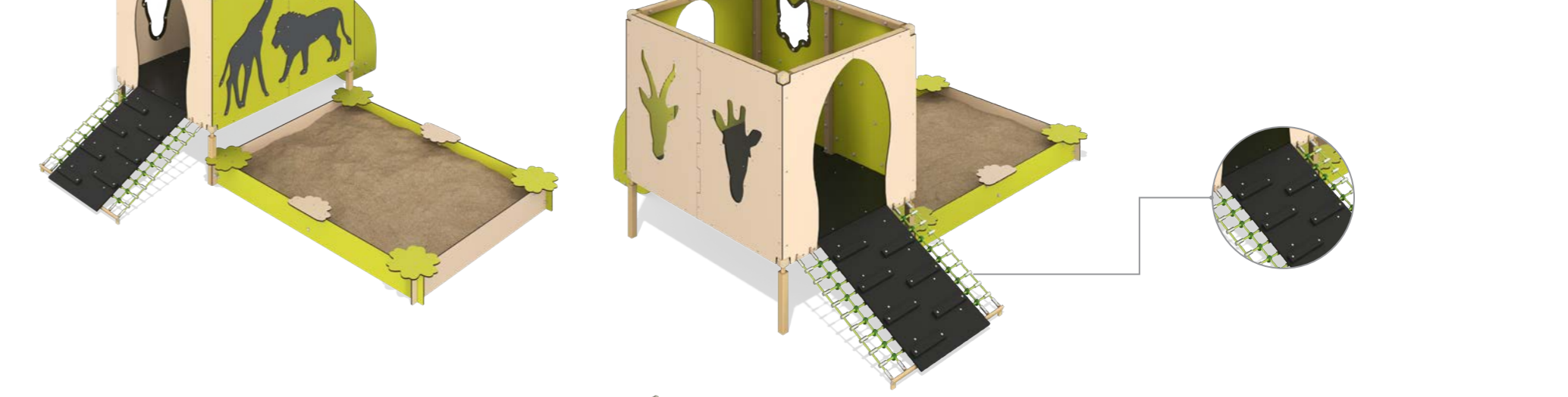
19.066 Sandpit Safari width length height fall height 4 000 mm 4 085 mm 1 960 mm 570 mm Age range: 3-12 years
